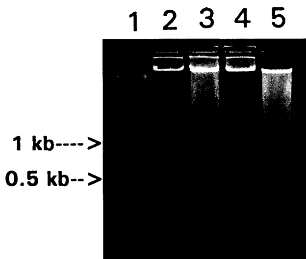
FIG. 6. Electrophoresis of genomic DNA from HCT-15 cells treated with sulindac sulfide, PGE 2 , and PGF 2α . Genomic DNA was isolated from HCT-15 cells and fractionated on 1.8% agarose gels, as described in Materials and Methods. HCT-15 cells treated with sulindac sulfide (200 μM) revealed the characteristic ladder pattern, a hallmark of apoptosis, which was not prevented by simultaneous addition of PGE 2 and PGF 2α at 10 -10 M. Lane 1 = molecular weight marker; lane 2 = control; lane 3 = sulindac sulfide, 200 μM; lane 4 = PGE 2 + PGF 2α ; and lane 5 = sulindac sulfide plus PGE 2 and PGF 2α .
