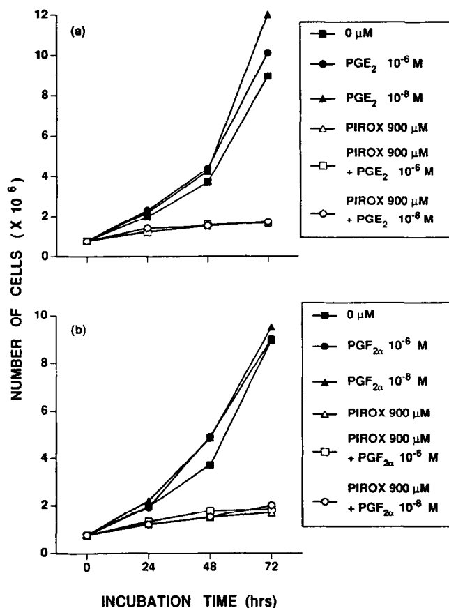
FIG. 3. Effects of piroxicam, PGE_2 , and PGF_{2\alpha} on cell proliferation in HCT-15 cells. Cells were cultured and counted at 24, 48, and 72 hr as described in Materials and Methods. Cells were treated with piroxicam (900 \mu M) with and without the addition of PGE_2 (a) or PGF_{2\alpha} (b), both at 10^{-6} and 10^{-8} M. Each number represents the mean of three separate experiments.
